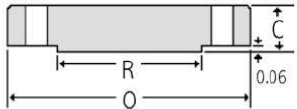
Blind
