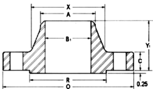
Weld Neck
