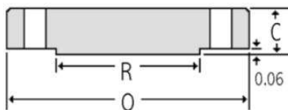
Blind
