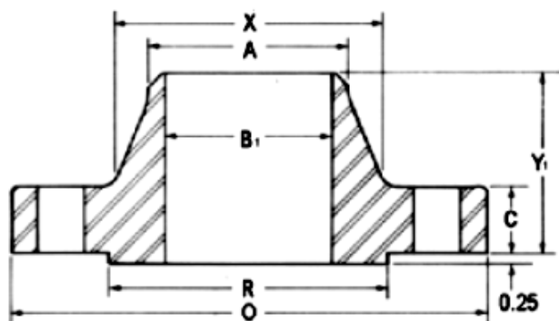
Weld Neck
