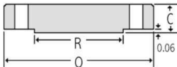
Blind
