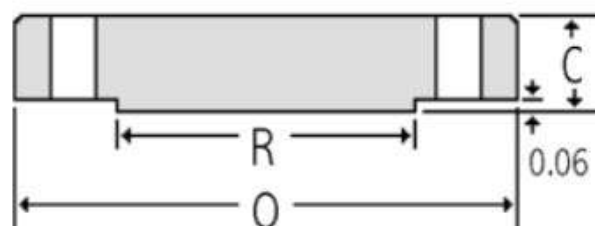
Blind
