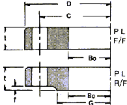
Plate
