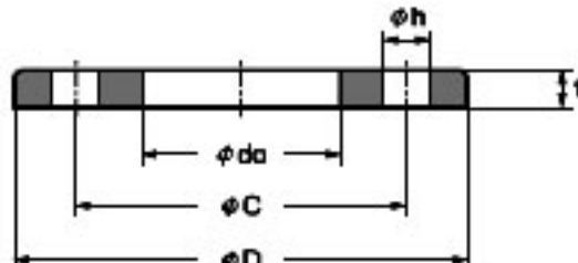
Slip-On
