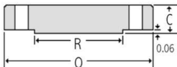
Blind
