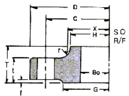
Slip-On
