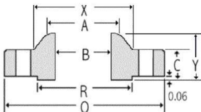
Weld Neck
